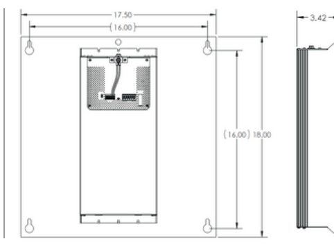
CEPS-250 with Wall Mount
