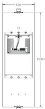
CEPS-125 with Grid Mount
