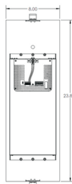
CEPS-250 with Grid Mount
