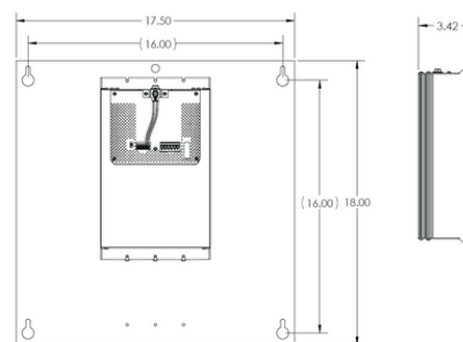
CEPS-125 with Wall Mount
